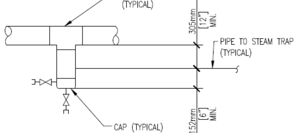
STEAM LINE DRIP POCKET
