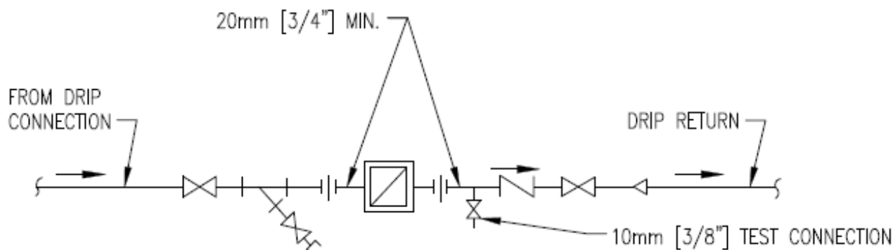
STEAM TRAP ASSEMBLY
