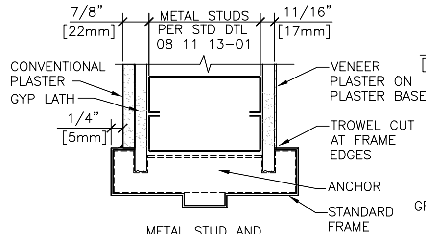
FRAMES WITH METAL STUD AND PLASTER PARTITIONS
