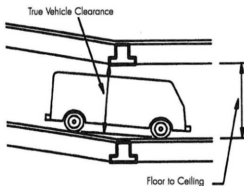
HEIGHT CLEARANCE
