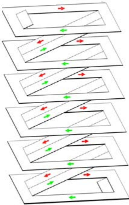
Side-by-Side Single-Helix
