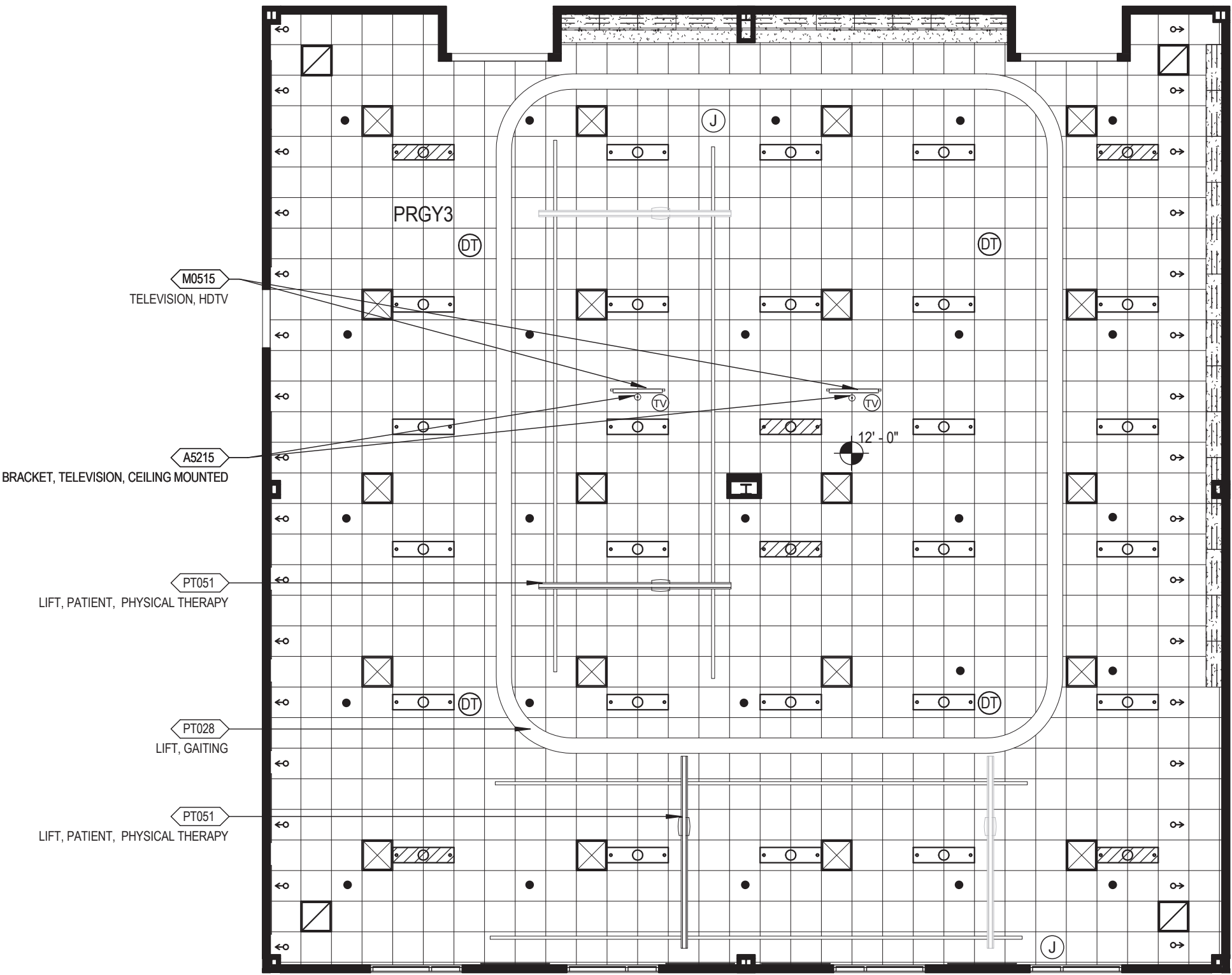
Polytrauma Rehabilitation Center • Outpatient Unit Reflected Ceiling Plan
