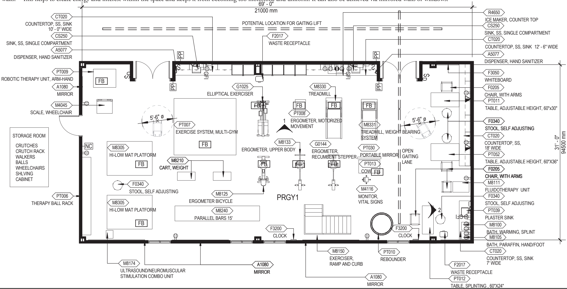
Polytrauma Rehabilitation Center • Inpatient Unit Floor/Equipment Plan (2,100 NSF/195.3 NSM)
