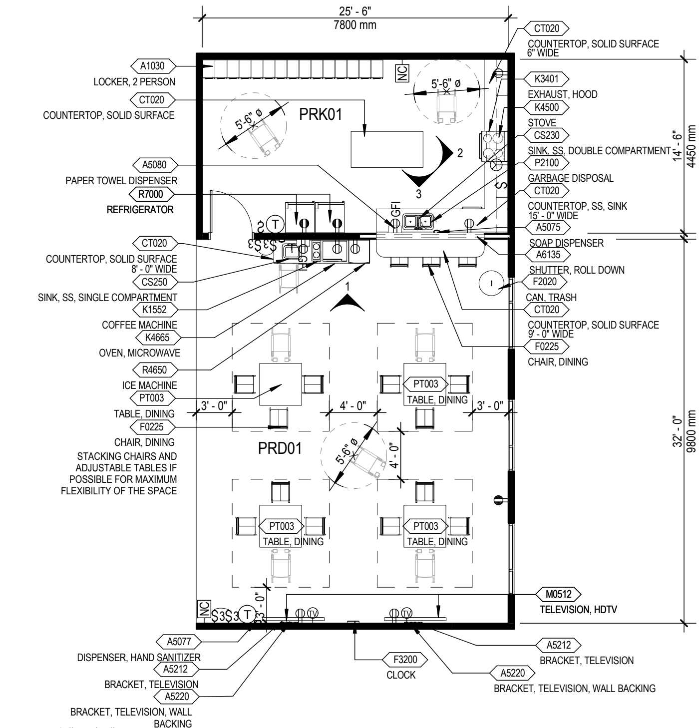
Polytrauma Rehabilitation Center • PTRP Floor/Equipment Plan (800 NSF/74.4 NSM; 360 NSF/33.5 NSM)
