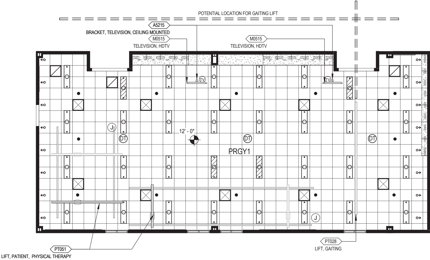
Polytrauma Rehabilitation Center • Inpatient Unit Reflected Ceiling Plan
